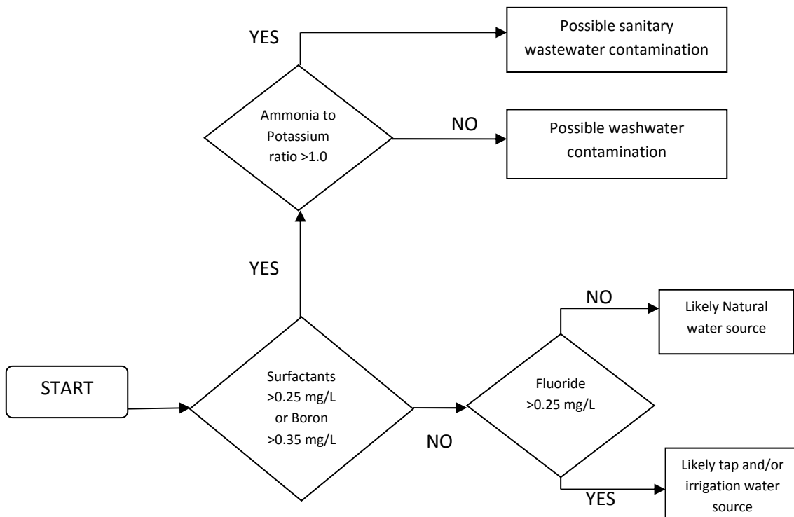
Figure 1: Flow Chart to Identify Illicit Discharges in Residential Watersheds (2004 IDDE Manual: Dr. Robert Pitt)
